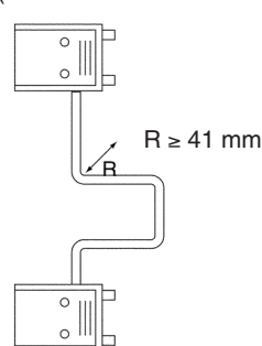
Cables for CS1 Long-distance Expansion Racks (Cable diameter: 10 mm)
