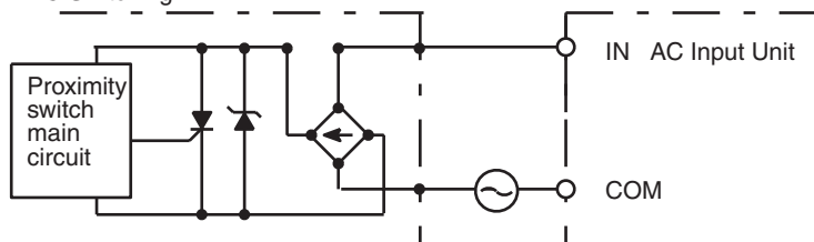
AC Switching
