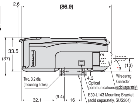
With Mounting Bracket Attached
