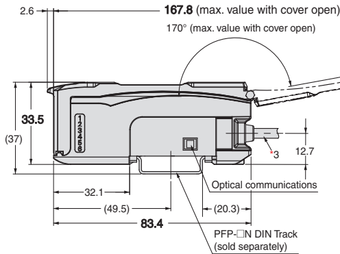
Mounted to DIN Track
