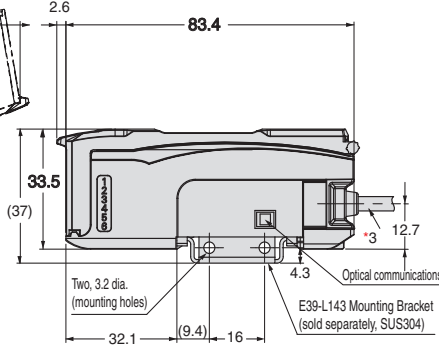
With Mounting Bracket Attached
