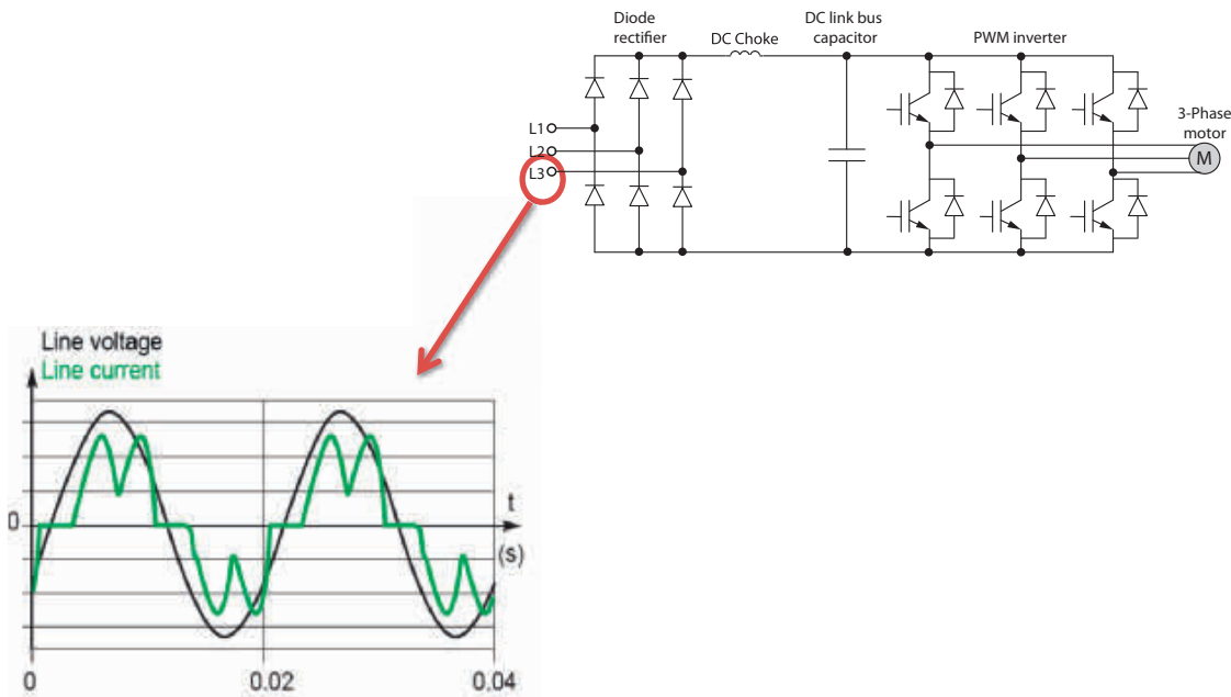
Fig. 3 Harmonic currents
