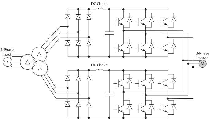
Fig. 9 18 pulse supply
