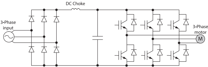
Fig. 7 DC-choke
