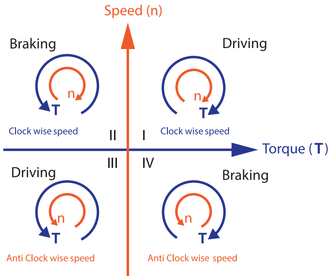
Fig. 10 4 Quadrant operation
