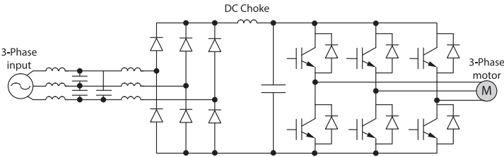
Fig. 8 12 pulse supply
