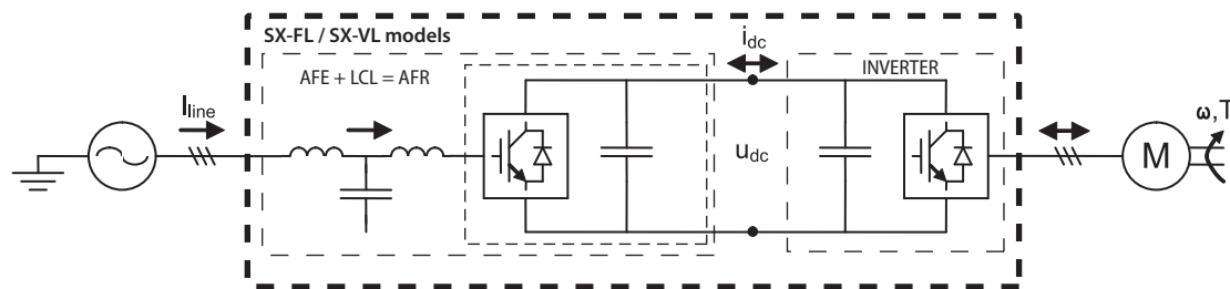
Fig. 14 Low harmonic
