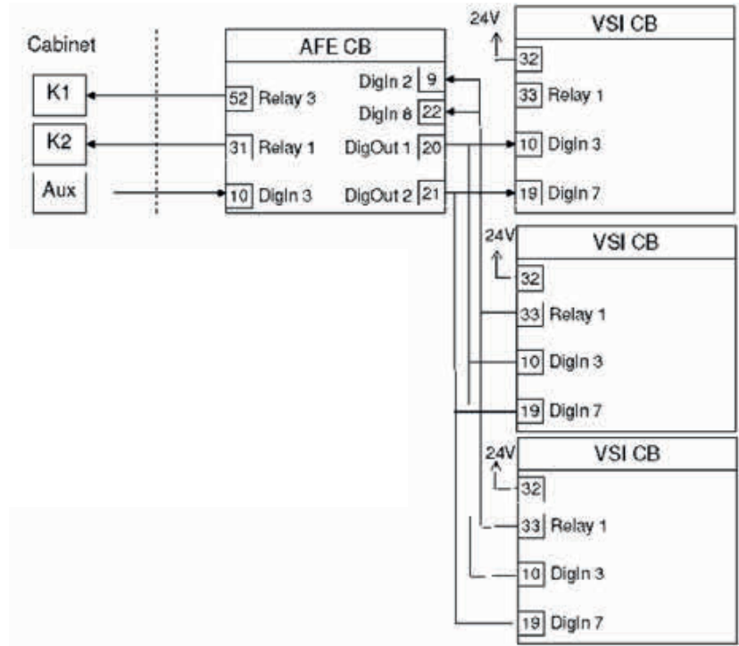
Fig. 20 Example of internal connections between AFR and VSI's
