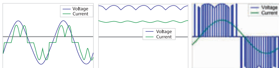
Fig. 12 DFE 6-pulse
