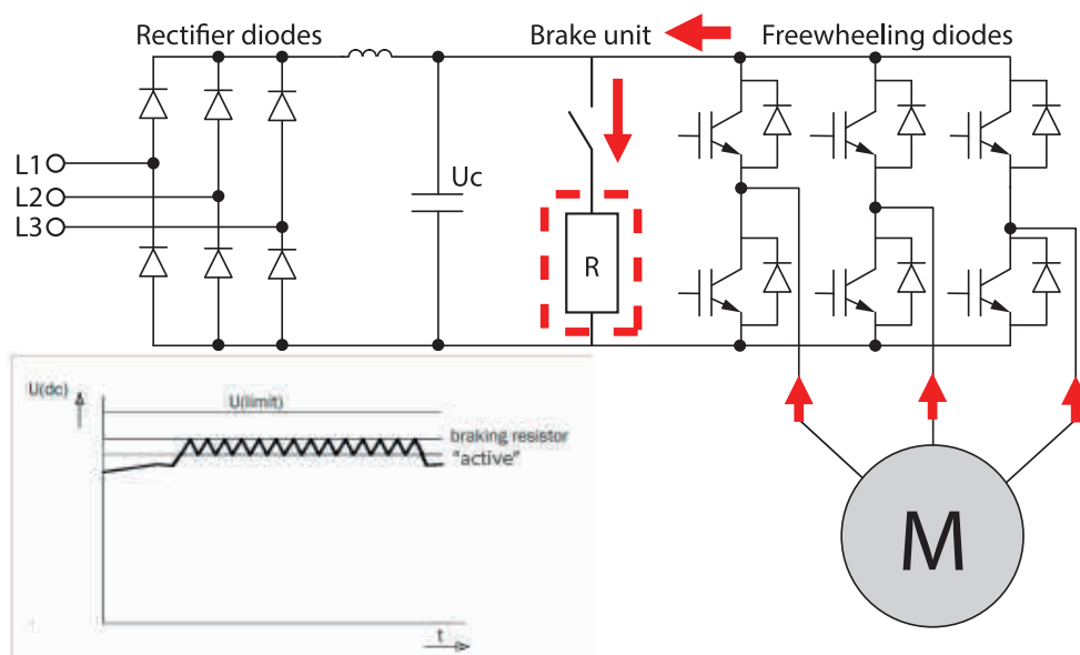
Fig. 11 Electrical braking
