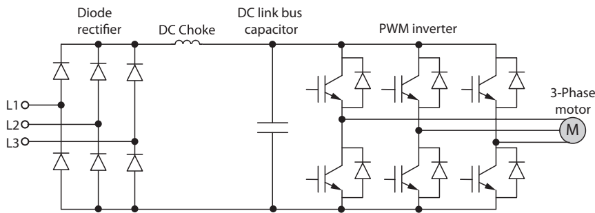
Fig. 1 6-pulse AC drive system
