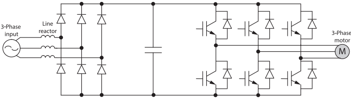
Fig. 6 Line reactor
