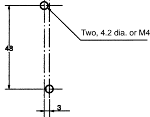
Mounting Holes
