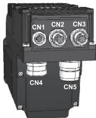
R88E-AECT0230/0330/ 0430/0530 models
