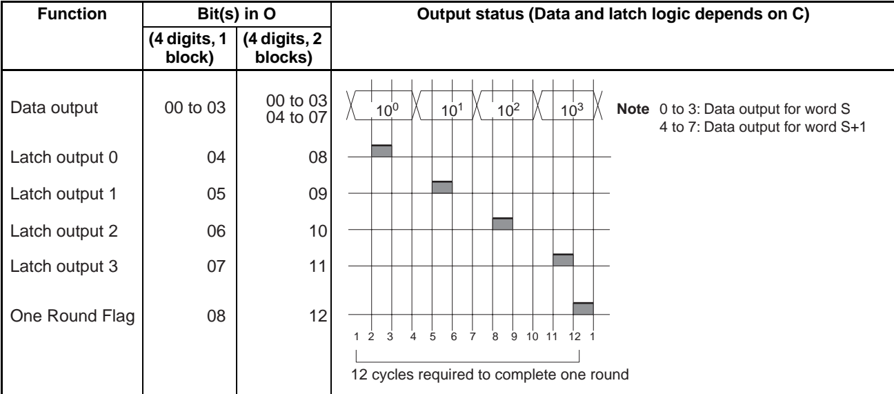
Timing Chart
