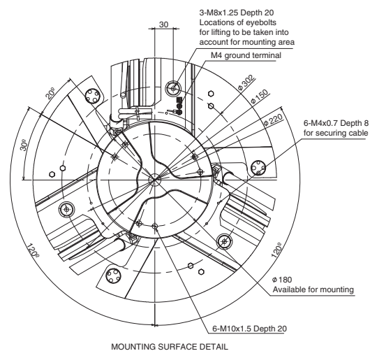
MOUNTING SURFACE DETAIL
