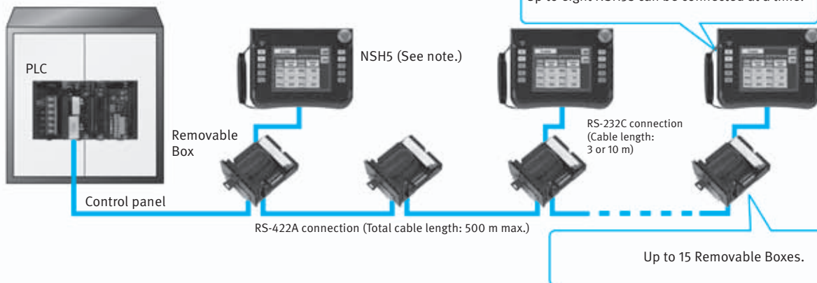
System Configuration (Removable Box Connected)
