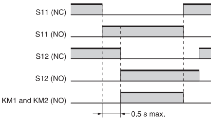
Timing Chart
